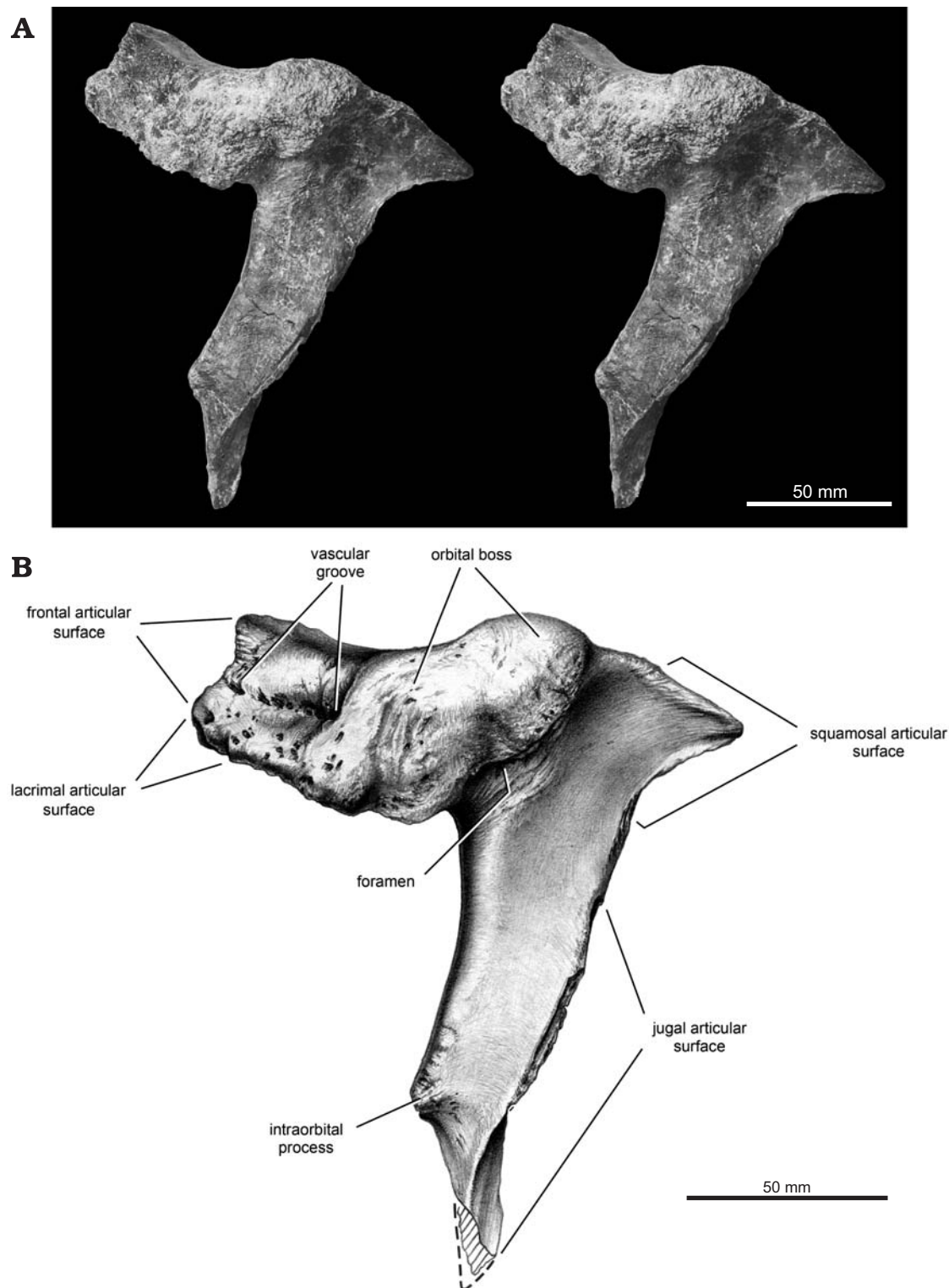
Fig. 9. Carcharodontosaurid theropod Eocarcharia dinops gen. et sp. nov. MNN GAD2 from the Lower Cretaceous Elrhaz Formation of Niger. Left postorbital (holotype) in lateral view; stereopair ( A ) and line drawing ( B ). Cross-hatching indicates broken bone; dashed lines indicate estimated edge.
