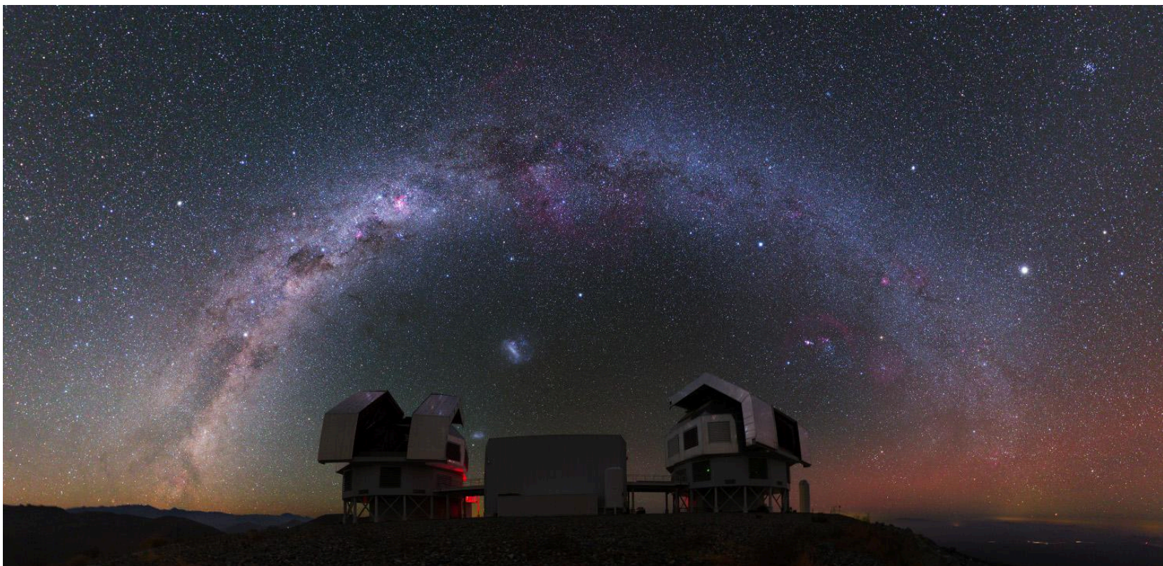
The Magellan Telescopes at Las Campanas Observatory (credit: Yuri Beletsky)
